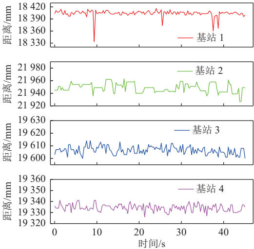
(a) 采煤机运动前的测量距离
