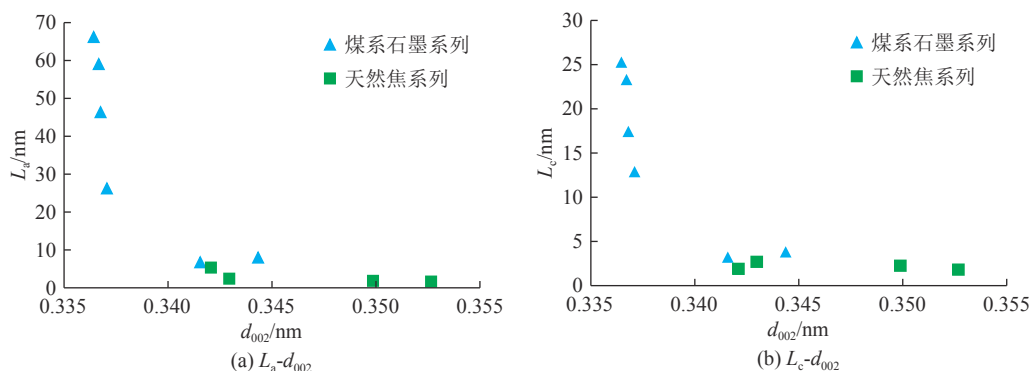
图3 XRD测试数据相关分析 Fig.3 Correlation analysis of XRD test data
