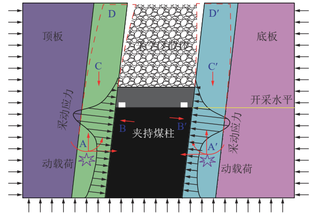
图 2 “夹持梁”力学模型 [32] Fig.2 “Clamping beam” mechanical model [32]
