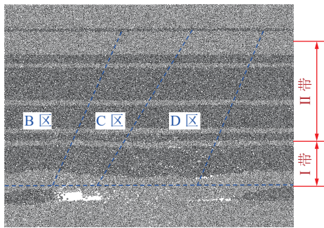
图 11 最终采场的不同区间微震事件破裂类型分布情况 Fig.11 Distribution of rupture types of microseismic events in different intervals of the final stope
