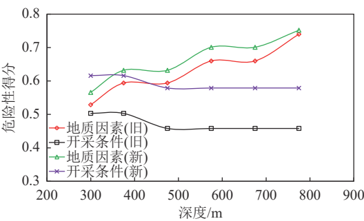
图 8 危险性得分随开采深度的变化 Fig.8 Variation of risk score with mining depth
