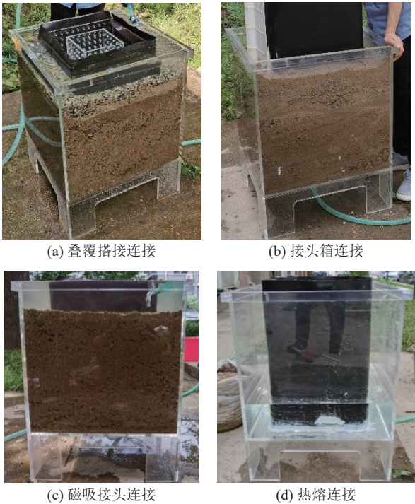
图 3 防渗膜接头连接工艺效果对比试验 Fig.3 Comparison test on the effect of anti-seepage membrane joint connection
